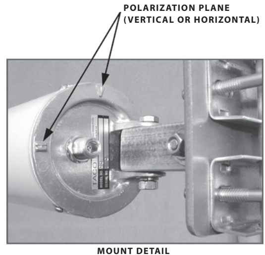
MOUNT DETAIL
